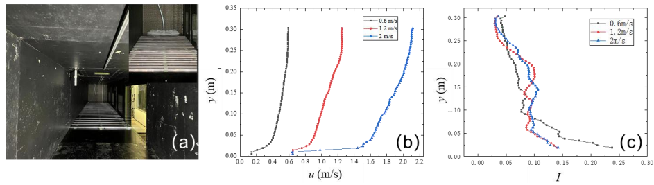
Figure 2-6 Roughness layout of wind tunnel (a) Average wind velocity profile (b) and turbulence intensity (c)
