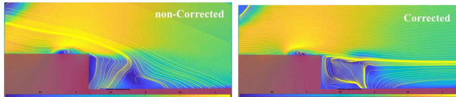
Figure 3-1 Comparison of time-averaged flow field in a large-scale cube
