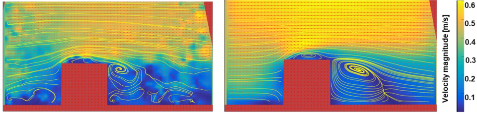
Figure 3-2 Instantaneous flow field and time-mean flow field of 1/20 cube
