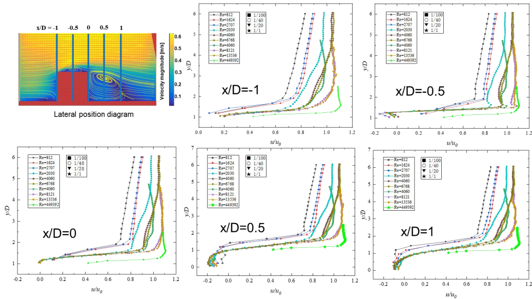
Figure 3-3 Comparison of longitudinal flow fields at different locations under different Reynolds numbers
