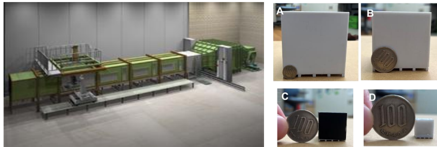
Figure 2-4 Temperature Stratification wind tunnel (left) and cube scale model (right)
