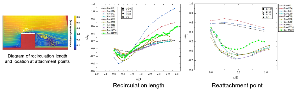
Figure 3-4 Comparison of top and tail flow fields under different Reynolds numbers
