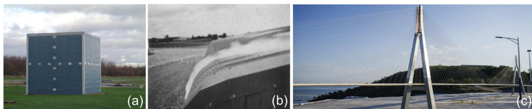
Figure 2-1 6 m cube in natural wind tunnel (a), building flow field measurement (b) and large-scale bridge measurement (c)
