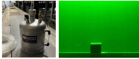
Figure 2-5 Oil drop generator (left) and 1/100 wind tunnel measurement (right)
