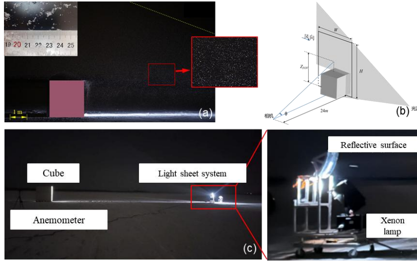
Figure 2-3 Actual shooting of cubes (a,b) and site layout (c)
