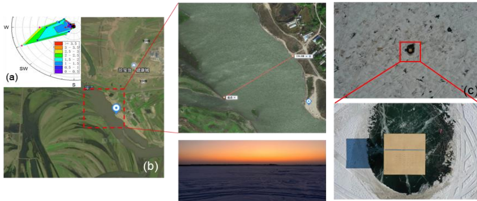
Figure 2-2 Wind speed and direction distribution (a), natural wind tunnel (b) and cube shooting (c) 2.2. Full scale field PIV measurement by snowflake tracer
