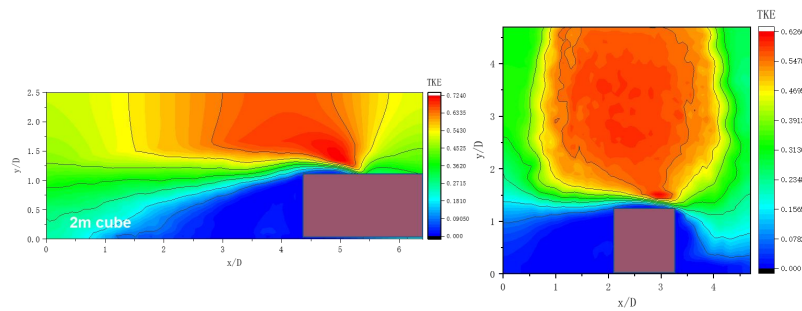
Figure 3-5 Comparison of dimensionless turbulent energy between a large-scale cube and a 1/20 scale cube
